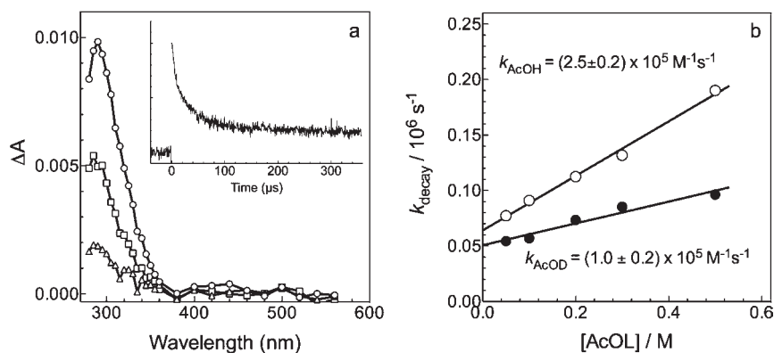
Figure 4. (a) Transient absorption spectra of a 0.14 mM solution of 4 in air-saturated THF, 0–1.3 \mu\text{s} (○), 19.8–22.4 \mu\text{s} (□), and 343–347 \mu\text{s} (△) after the laser pulse; the inset shows a transient decay profile recorded at 290 nm. (b) Plots of k_{\text{decay}} vs [\text{AcOL}] ( L = \text{H} or \text{D} ) for quenching of the 290 nm species by AcOH and AcOD in air-saturated hexane at 25 °C.
